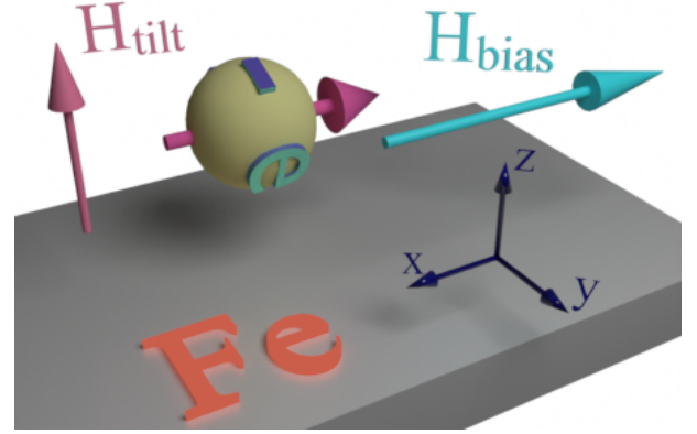
FIG. 1. Ferromagnetic iron film with in-plane magnetic anisotropy: geometry. The green ball shows the equilibrium spin direction along the easy axis, which is oriented in the film plane (along the x-axis). The strength of the magnetic anisotropy is probed by applying a tilt field H_{tilt} perpendicular to the equilibrium spin direction and the film plane (along the z- axis). The field H_{tilt} forces the spins to tilt away from the easy axis towards the film normal; the stronger the magnetic anisotropy, the larger the value of H_{tilt} required to achieve the same tilt angle. A bias magnetic field H_{bias} is applied along the easy axis (the x-axis) to enhance the effective anisotropy field.
